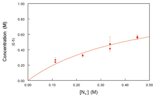
FIGURE 7. Yield of 5c obtained from the reaction of 4c at pH 7.0 and 50 °C as a function of [N 3 – ]. Data were fit to eq 5.
