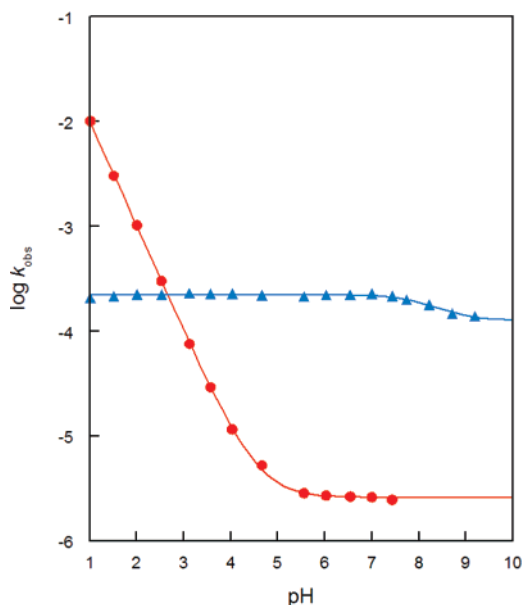
FIGURE 2. Log k_{\text{obs}} vs pH for 2c (red circles) and 4c (blue triangles). Data for 2c were obtained at 30 °C; data for 4c were obtained at 50 °C. Data were fit as described in the text.
