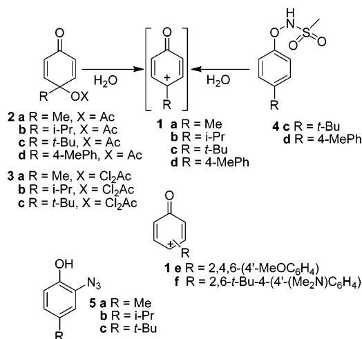
SCHEME 1. Possible Routes to 4-Alkylaryloxenium Ions
