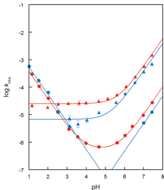
FIGURE 1. Log k_{\text{obs}} vs pH for 2a (red circles), 2b (blue circles), 3a (red triangles), and 3b (blue triangles). Data for 2a and 3a were obtained at 80 °C; data for 2b and 3b were obtained at 30 °C. Data were fit as described in the text.
