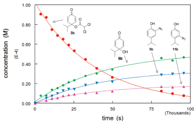
FIGURE 5. Formation of 5b , 6b , and 11b from 3b in 0.25 \text{ M } N_3^- at pH 4.5 and 30^\circ\text{C} monitored by HPLC. Data were fit to the first-order rate equation for all compounds.
