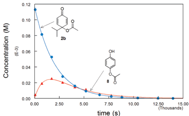
FIGURE 3. Formation and decay of 8 during decomposition of 2b at pH 1.0 and 80^\circ\text{C} . Concentration vs time data were fit to the first-order rate equation for 2b and the consecutive first-order rate equation for 8 : k_{\text{obs}} = (4.8 \pm 0.1) \times 10^{-4} \text{ s}^{-1} for 2b ; k_1 = (3.8 \pm 0.6) \times 10^{-4} \text{ s}^{-1} and k_2 = (9.3 \pm 1.7) \times 10^{-4} \text{ s}^{-1} for 8 .
