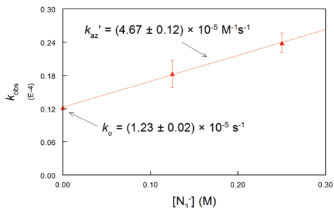
FIGURE 4. Plot of k_{\text{obs}} vs [N_3^-] for the decomposition of 3b in 1/1 N_3^-/\text{HN}_3 buffers at pH 4.5 and 30^\circ\text{C} . Rate constants were determined from HPLC data.
