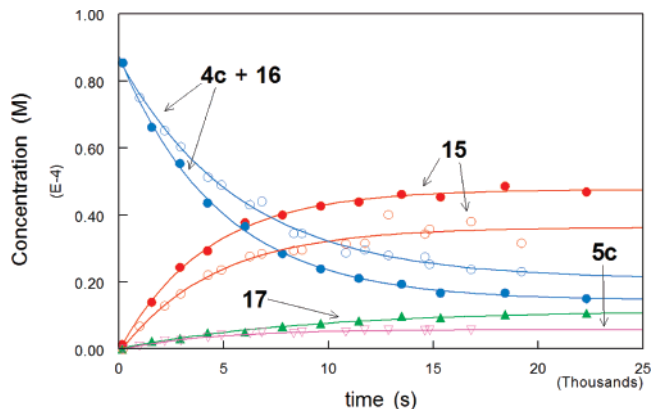
FIGURE 6. Concentration of products vs time during the decomposition of 4c at pH 7.0 and 50 °C in the presence of 0.45 M N 3 – (open symbols) and in its absence (solid symbols).
