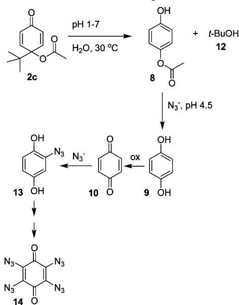
SCHEME 4. Products of the Decomposition of 2c
